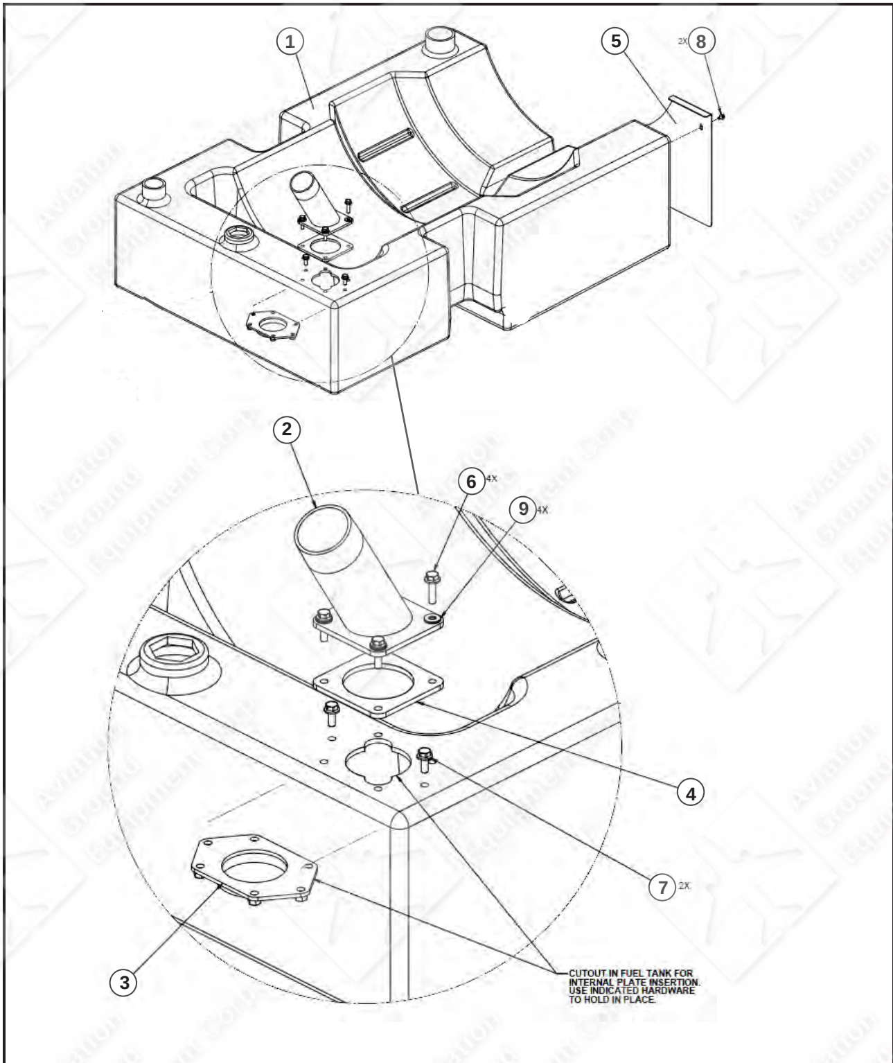
Figure 3-5. Fuel Tank Composite Assembly, 60-90 kVA (Sheet 1 of 2).
