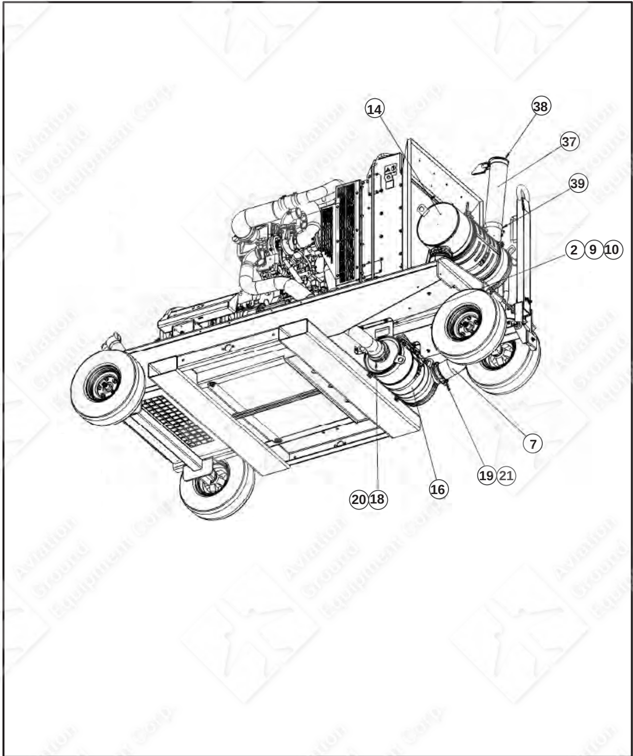
Figure 3-6. Radiator/After-Treatment Installation, 60-90 kVA (Sheet 3 of 4).
