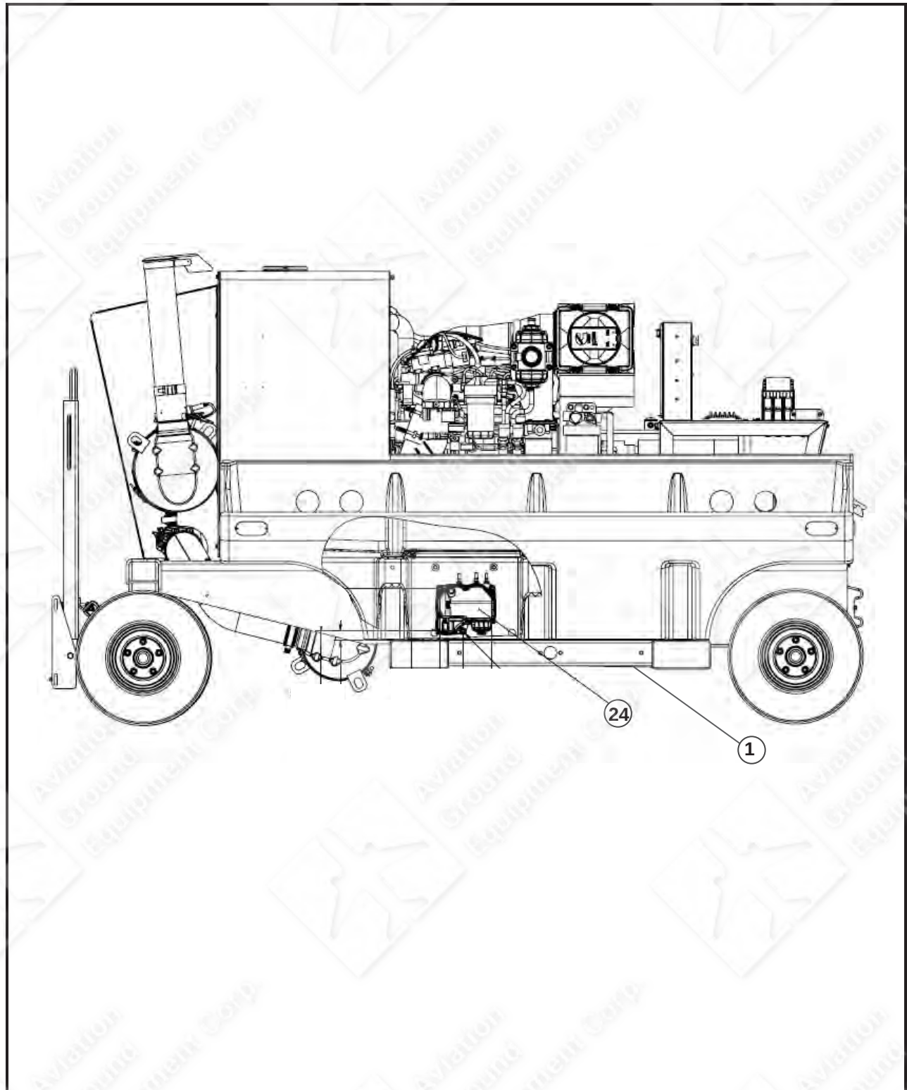
Figure 3-1. 4400-T4, 60-90 kVA, Generator Set (Sheet 3 of 5).
