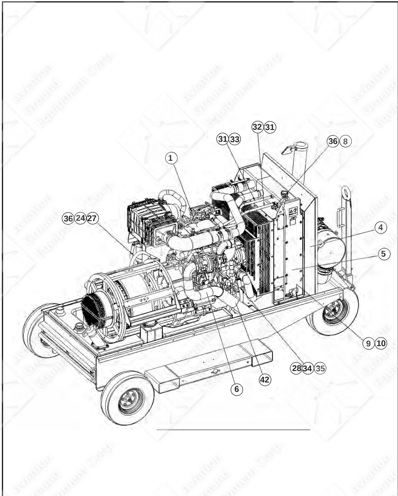
Figure 3-6. Radiator/After-Treatment Installation, 60-90 kVA (Sheet 1 of 4).
