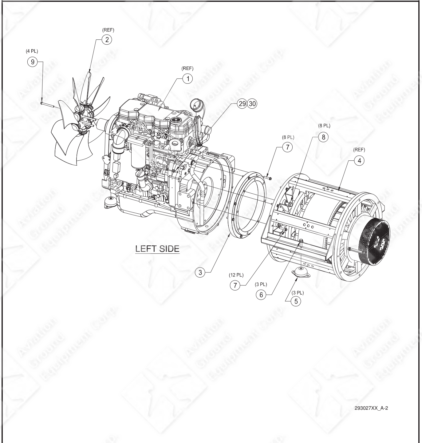
Figure 4-5. Genset Assembly, 60/90kVA (Sheet 1 of 4).
