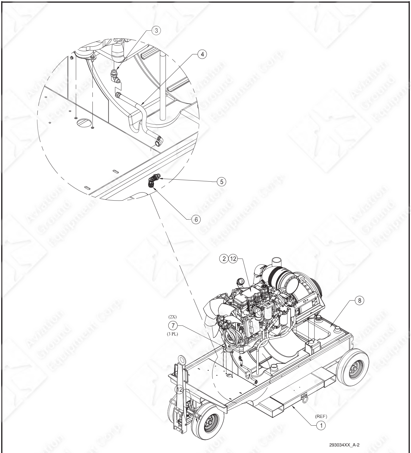
Figure 4-4. Genset/Fuel Tank Installation, 60/90 kVA (Sheet 2).
