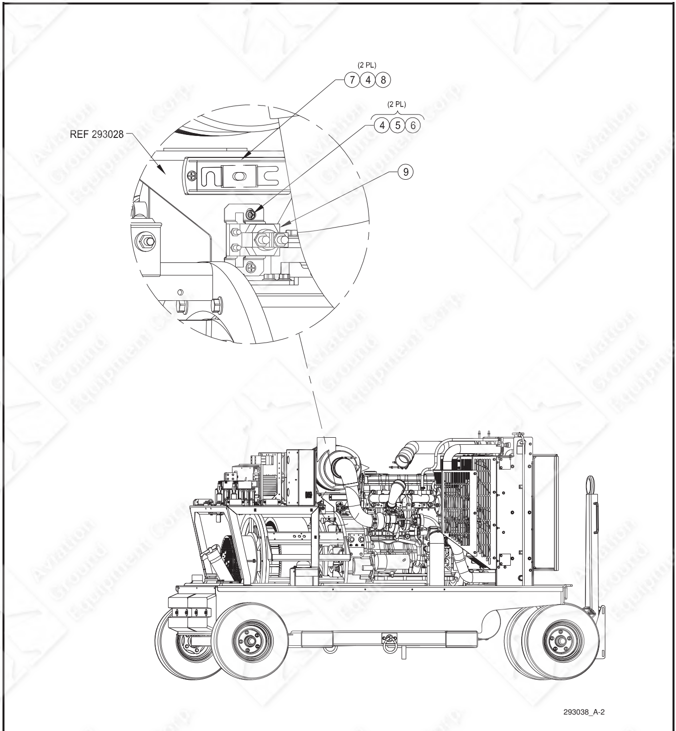
Figure 4-9. Electrical System Installation, 4400 (Sheet 2)
