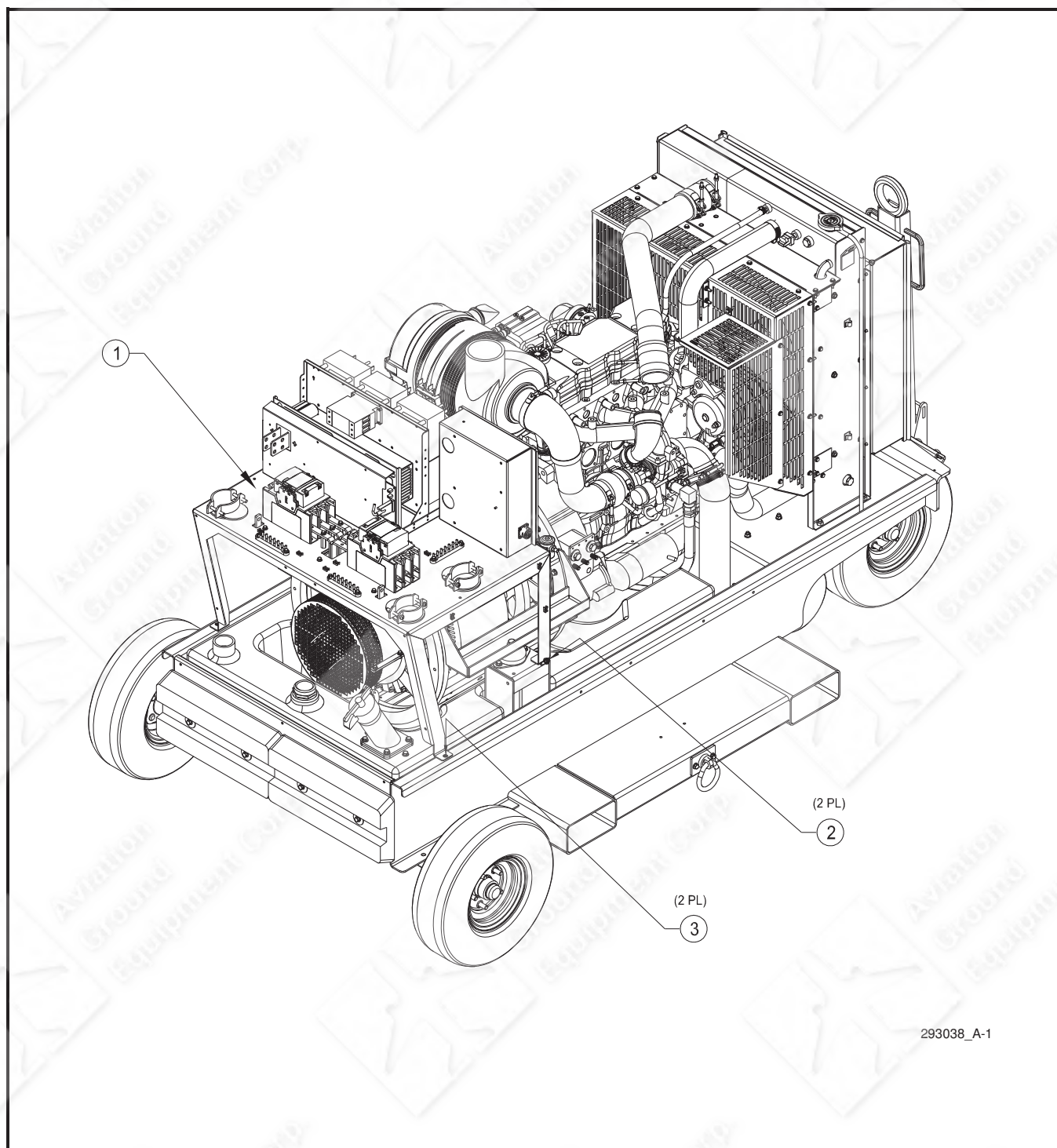
Figure 4-9. Electrical System Installation, 4400 (Sheet 1 of 3)
