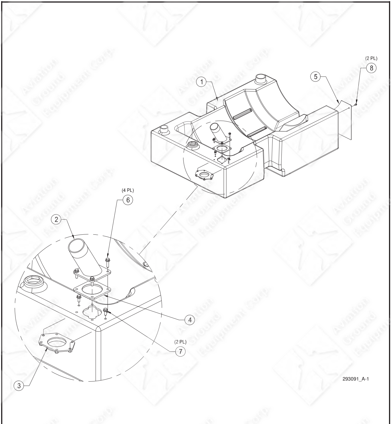
Figure 4-6. Fuel Tank Composite Assembly, CP (Sheet 1 of 2).
