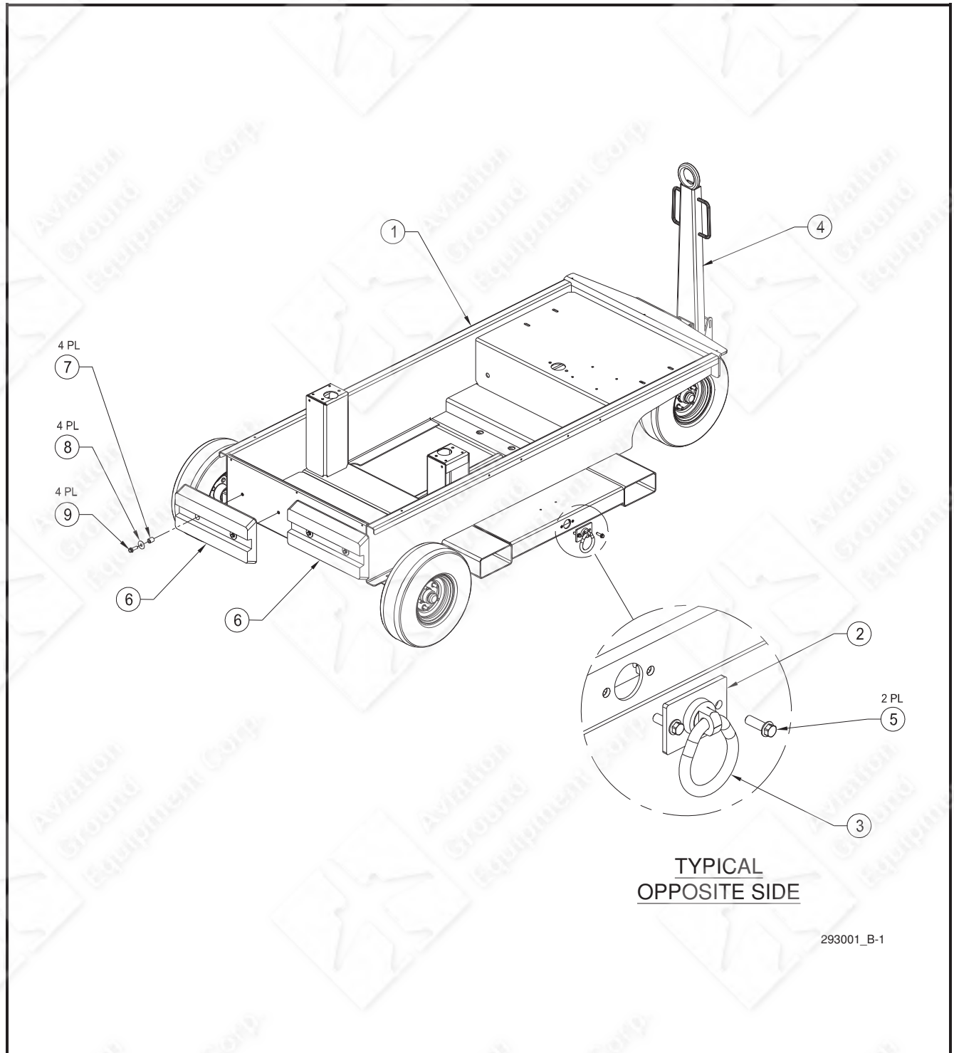
Figure 4-2. Trailer Assembly Common Platform (Sheet 1 of 2).
