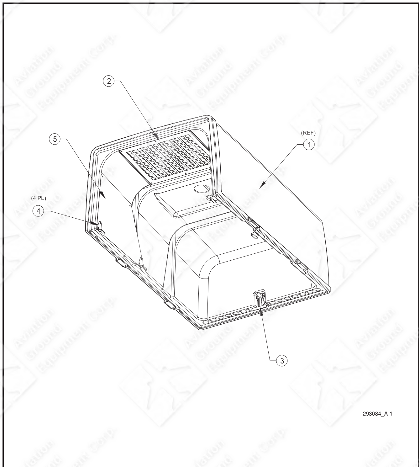
Figure 4-19. Top Canopy, Composite, Assembly (Sheet 1 of 2).
