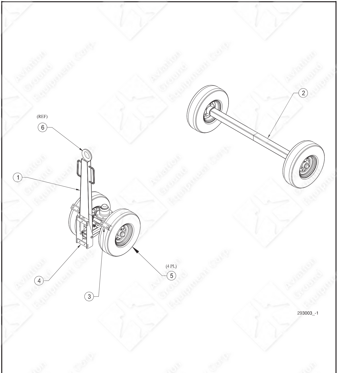
Figure 4-3. Running Gear Assembly, 4400 Platform. (Sheet 1 of 2).
