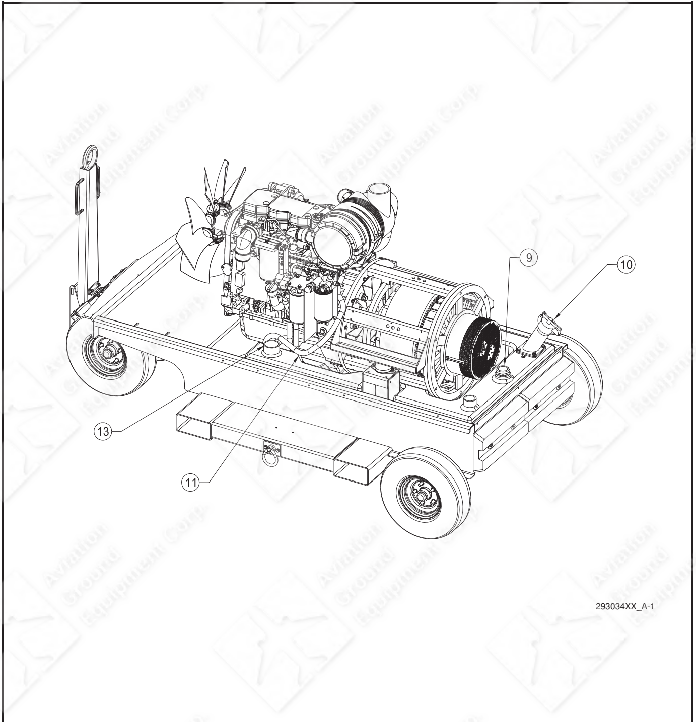
Figure 4-4. Genset/Fuel Tank Installation, 60/90 kVA (Sheet 1 of 3).
