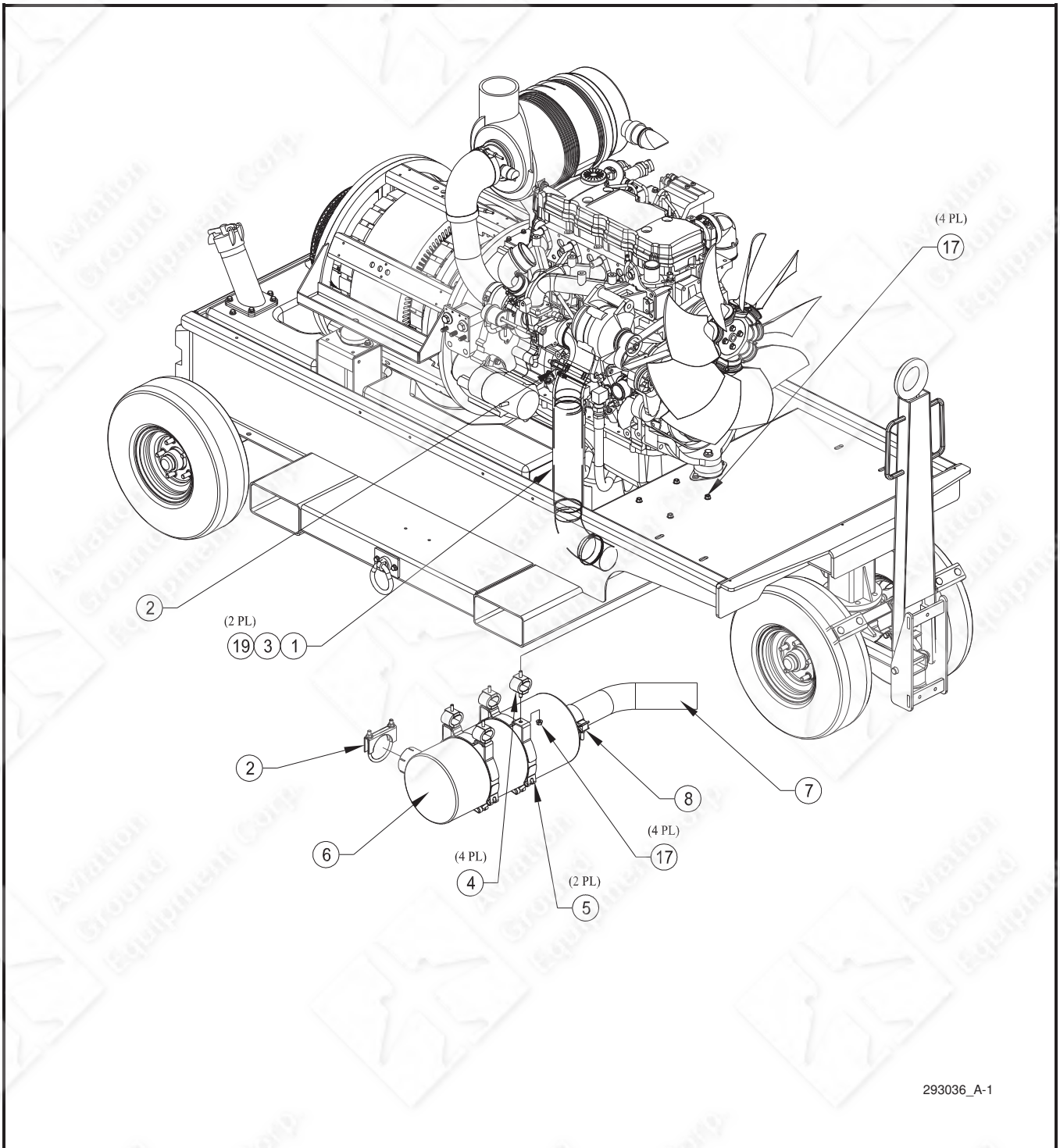
Figure 4-7. Radiator/Exhaust Installation (Sheet 1 of 3).
