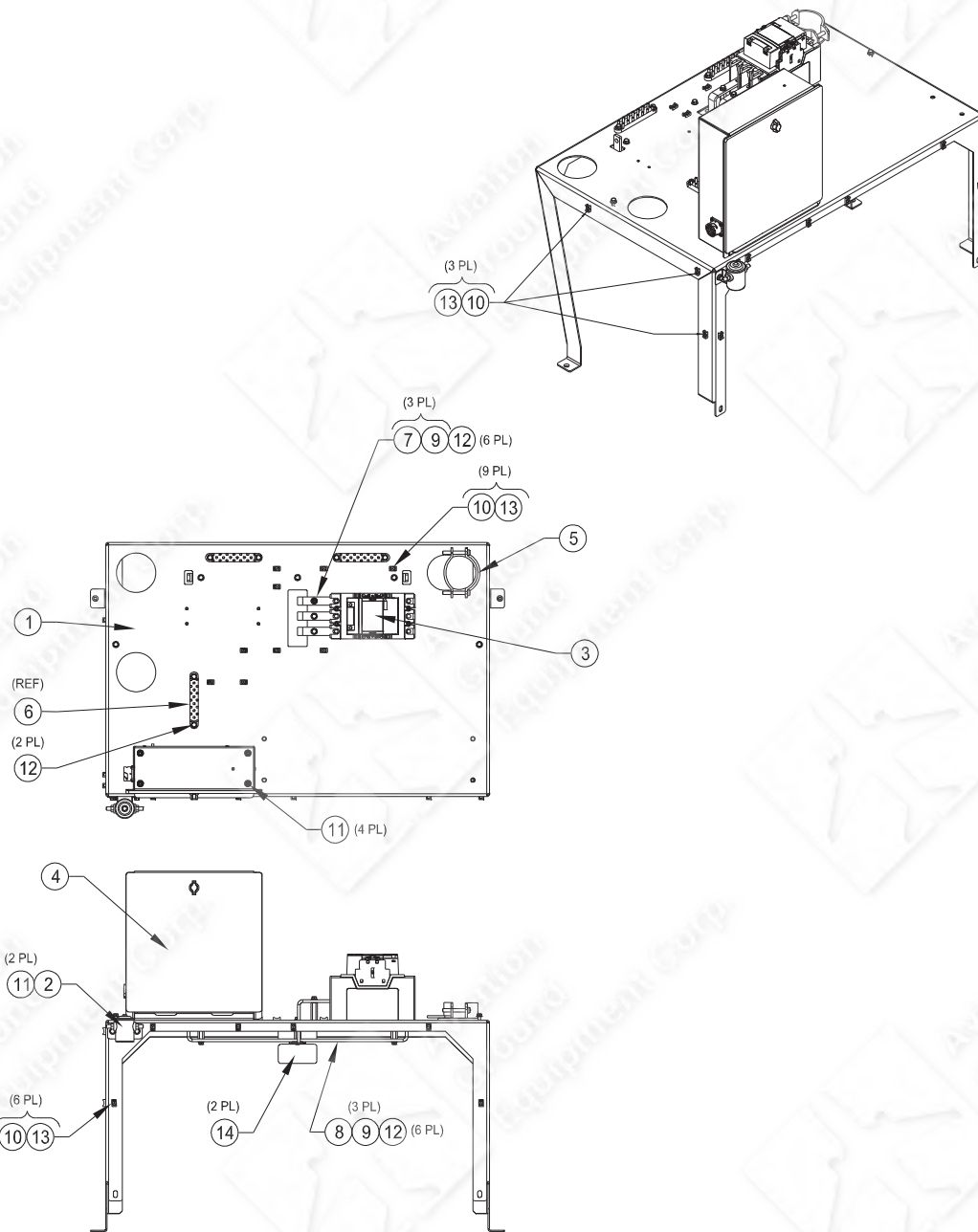
SINGLE OUTPUT, 4400 293039-01 CONFIGURATION
