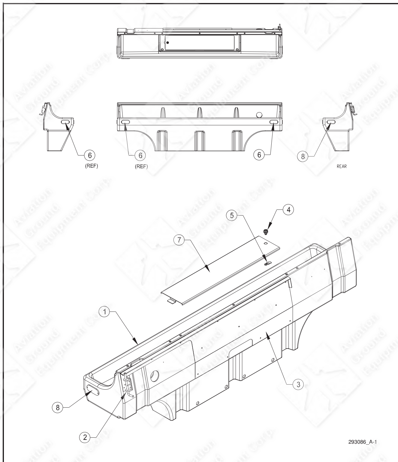
Figure 4-16. Cable Tray Assembly, Left Side (Sheet 1 of 2).
