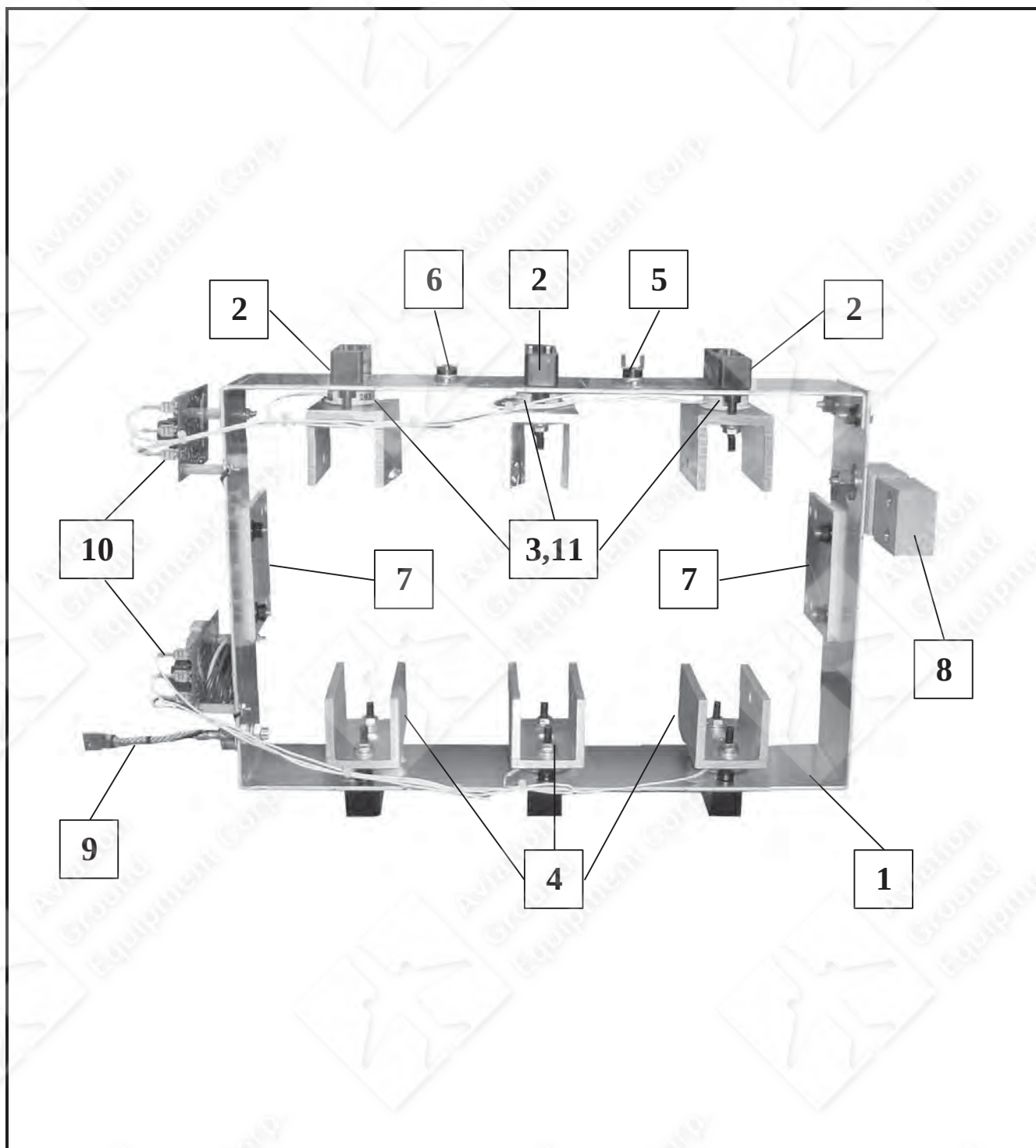
Figure 7 SCR Output Rectifier Assembly of GPU-400 Power Supply
