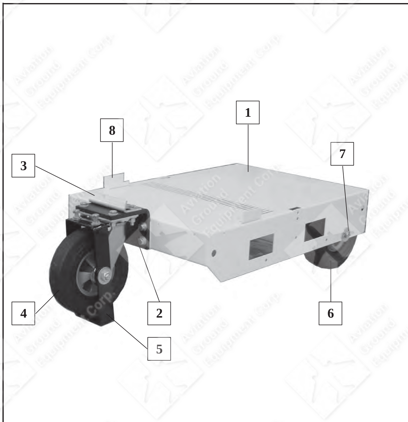
Base Assembly Figure 4
